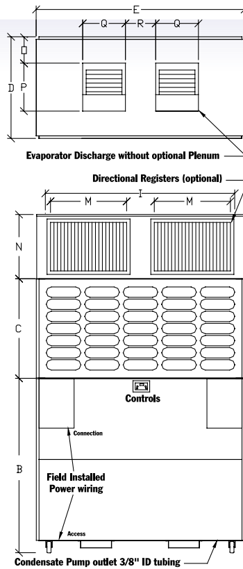
Condensate Pump outlet 3/8" ID tubing
